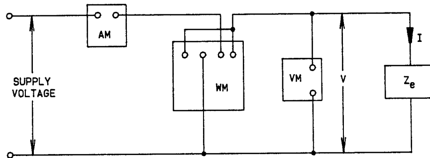
Figure 5-1—Method of Determining the Impedance
