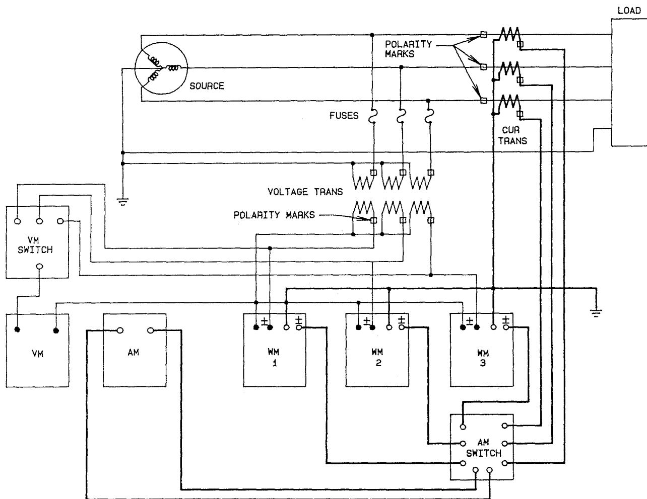
Figure 2-11—Transformer Connections for Measurement of a 3-Phase, 4-Wire (Circuit)
