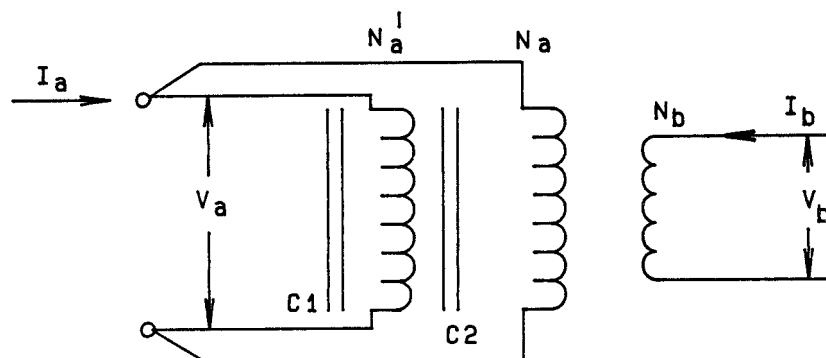
Windings N_a and N_b are placed on both cores, C1 and C2; windings N_a , having the same number of turns as N_a , is placed only on core C1.
