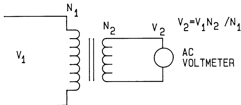
Figure 2-3—Measurement of High Alternating Voltages with a High Transformer
