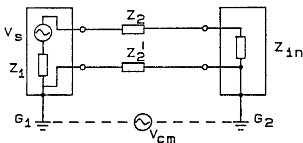
Figure 1-2—Common-Mode Voltage
